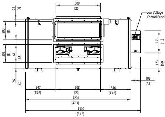
LEFT VIEW
