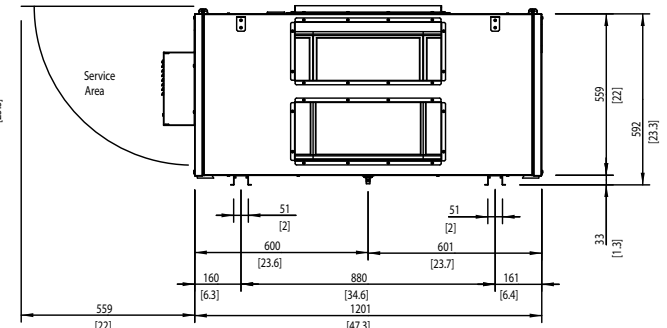
RIGHT VIEW
